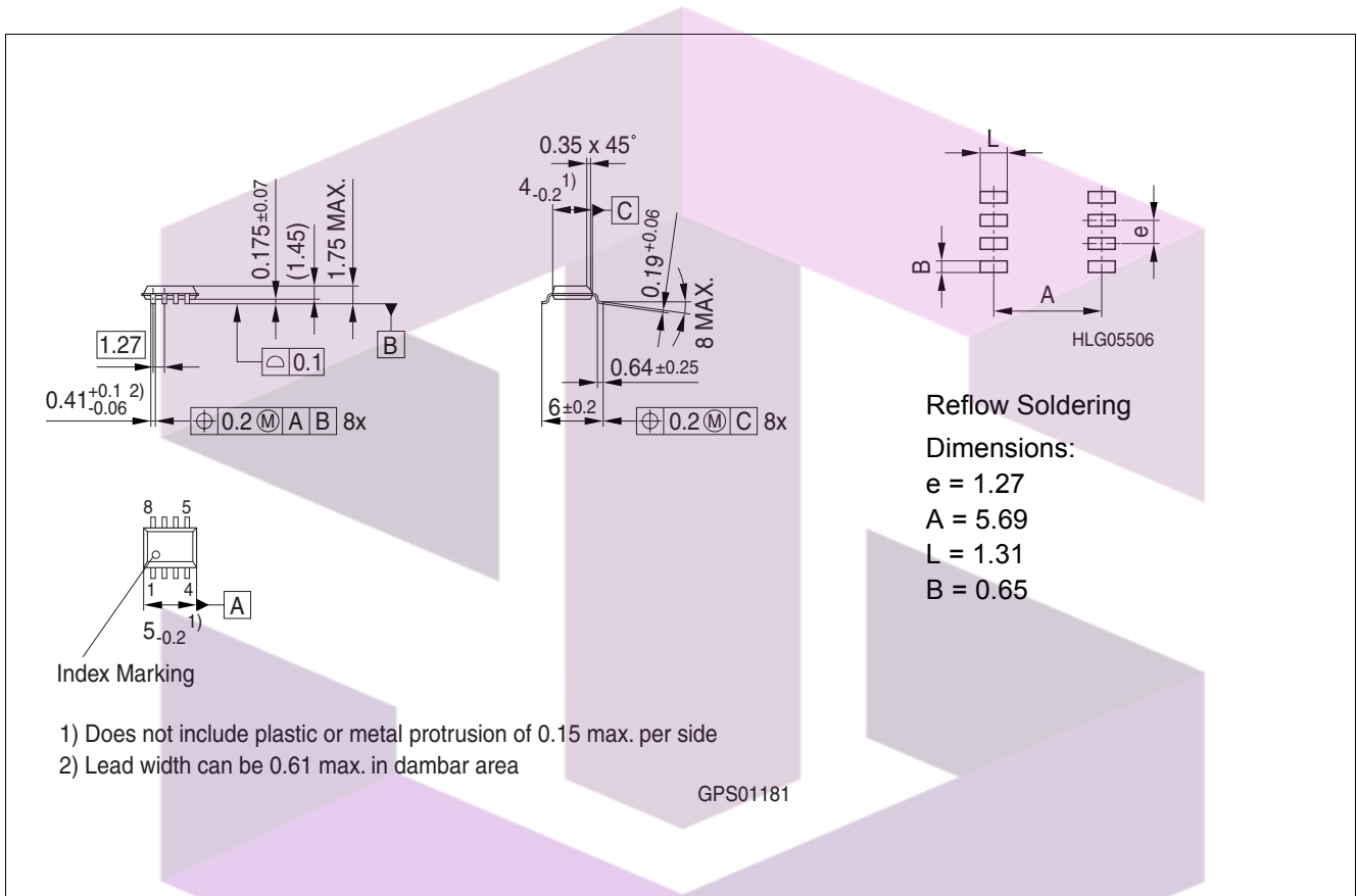
Figure 8 Outline and footprint PG-DSO-8
